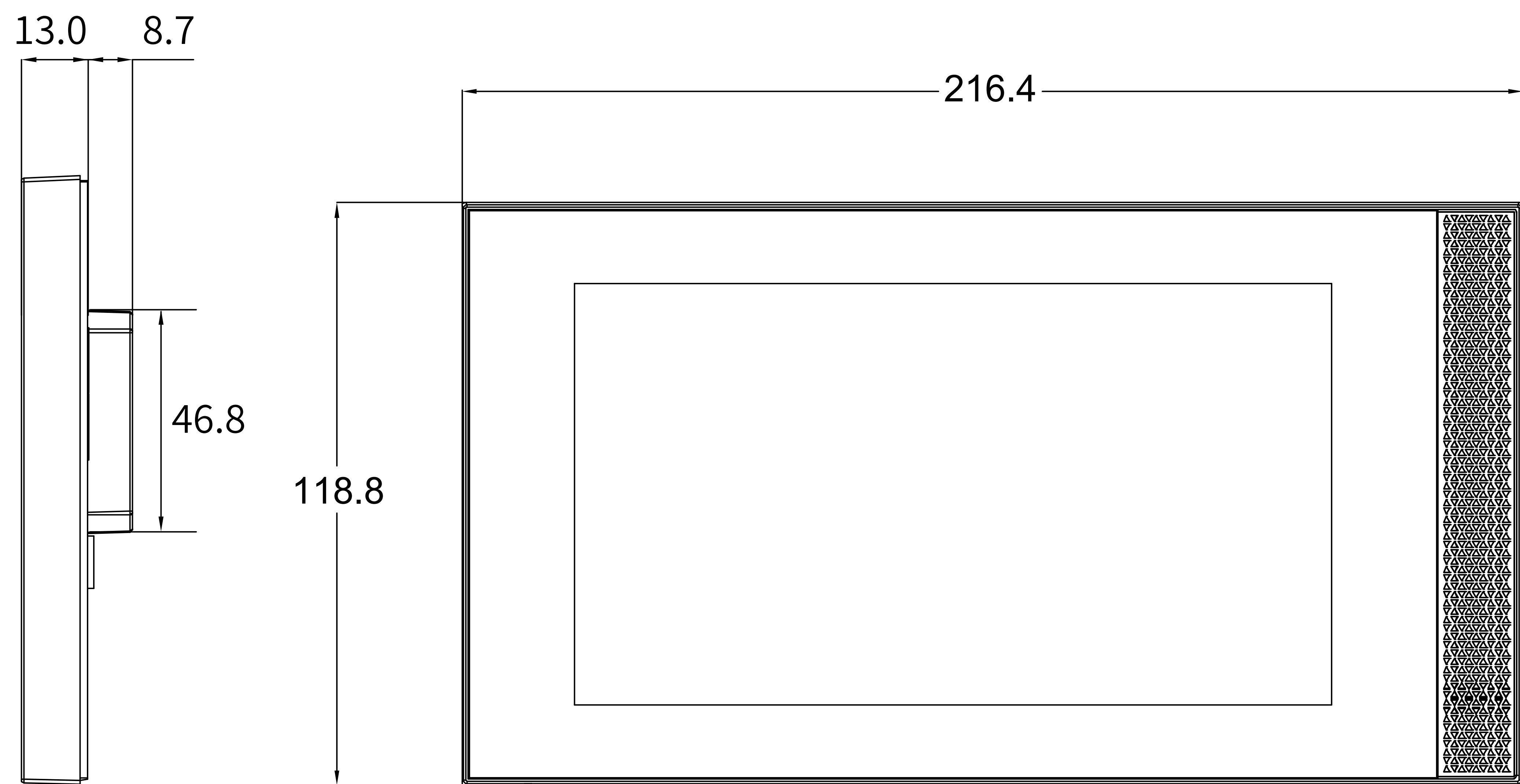
1 FRONT VIEW
