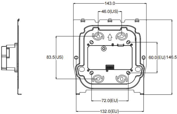
3 LEFT VIEW
