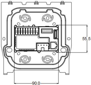
4 BACK VIEW
