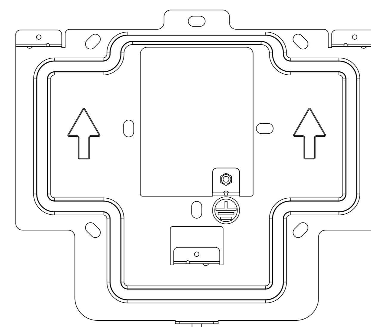
② FRONT VIEW:WALL MOUNTING BRACKET PLACEMENT
