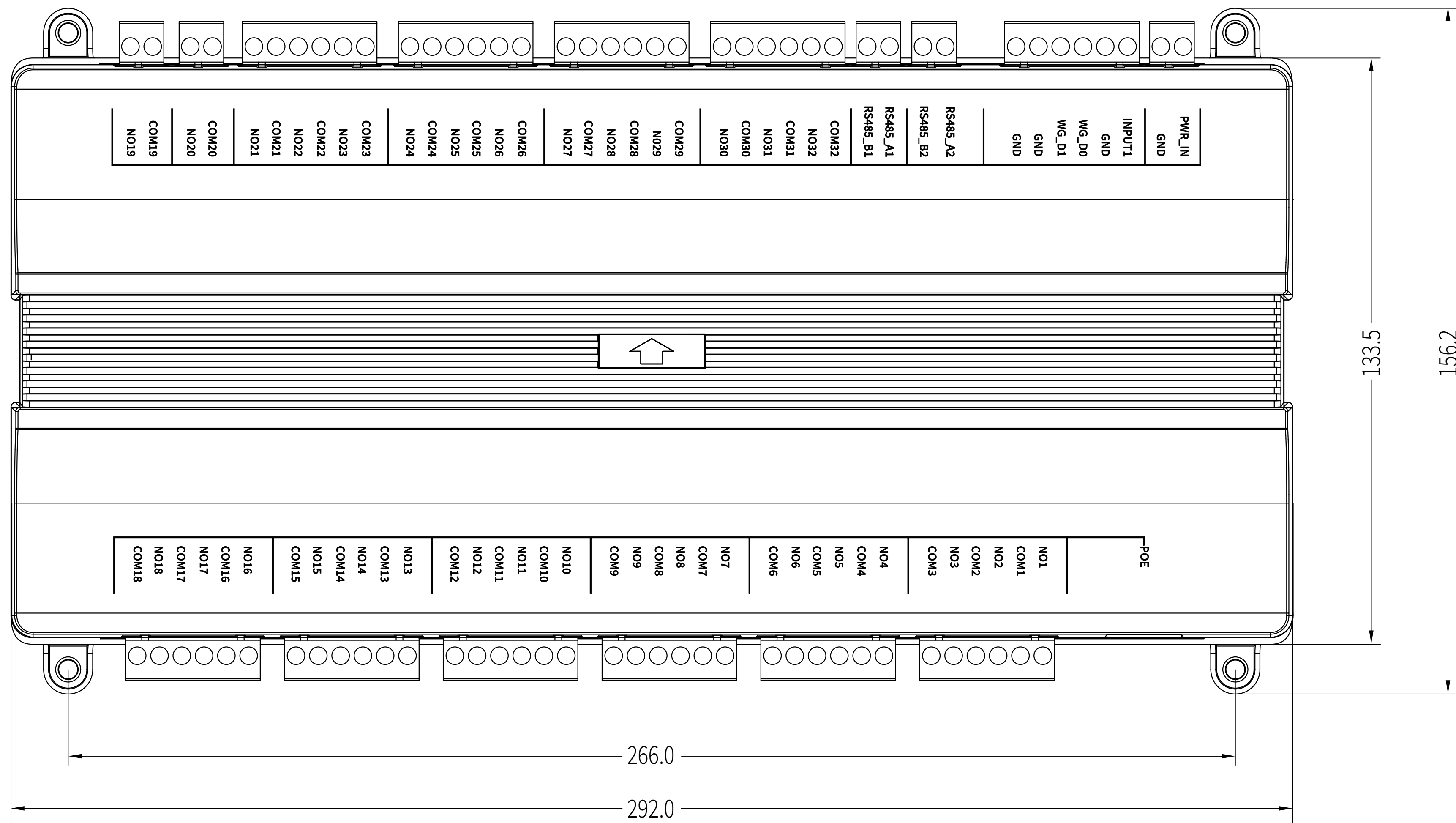
1 FRONT VIEW
