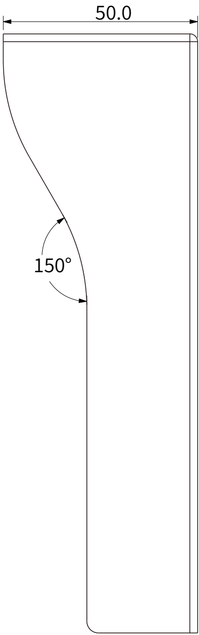
2 RIGHT VIEW
