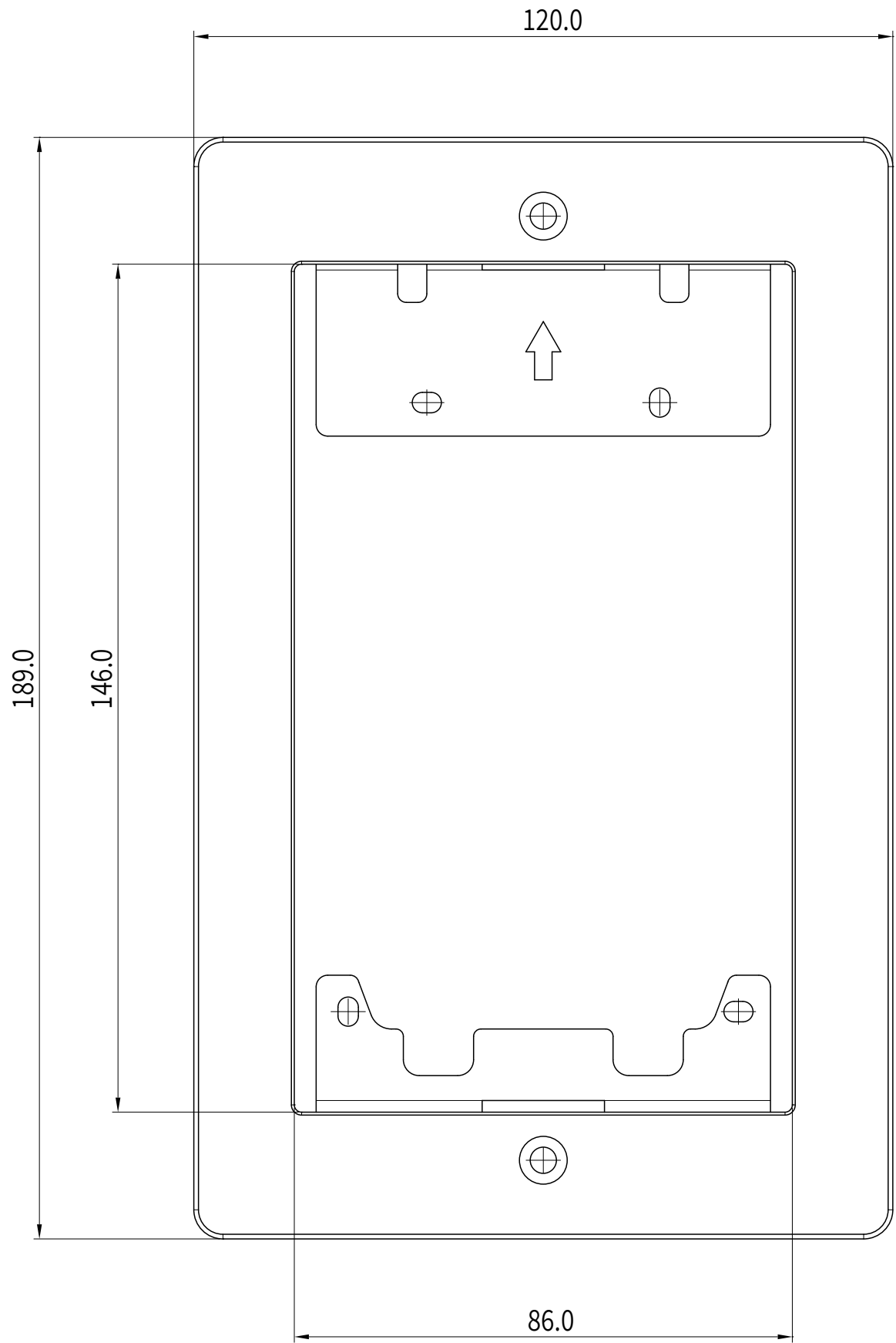
1 FRONT VIEW
