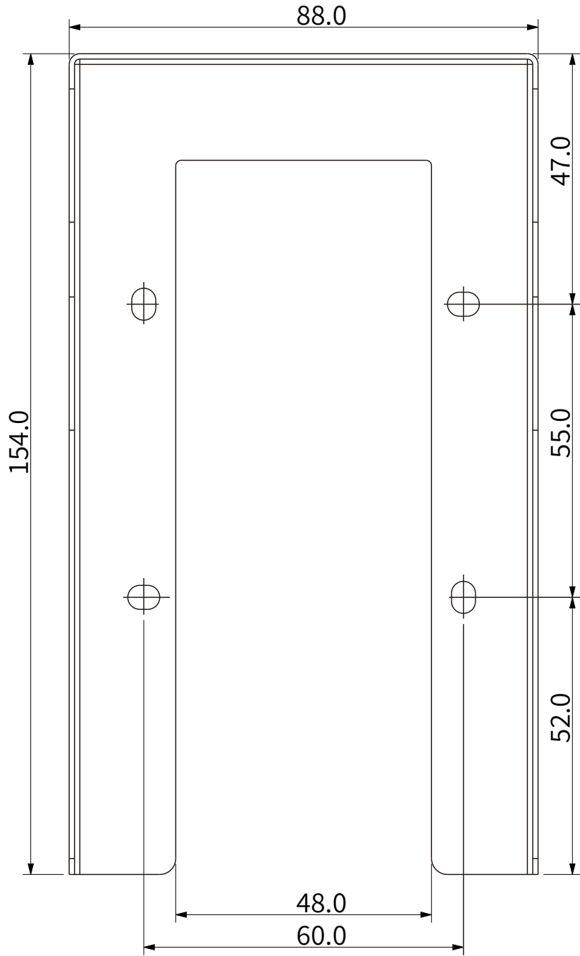
1 FRONT VIEW
