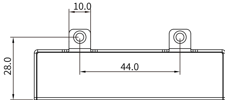
5 TOP VIEW
