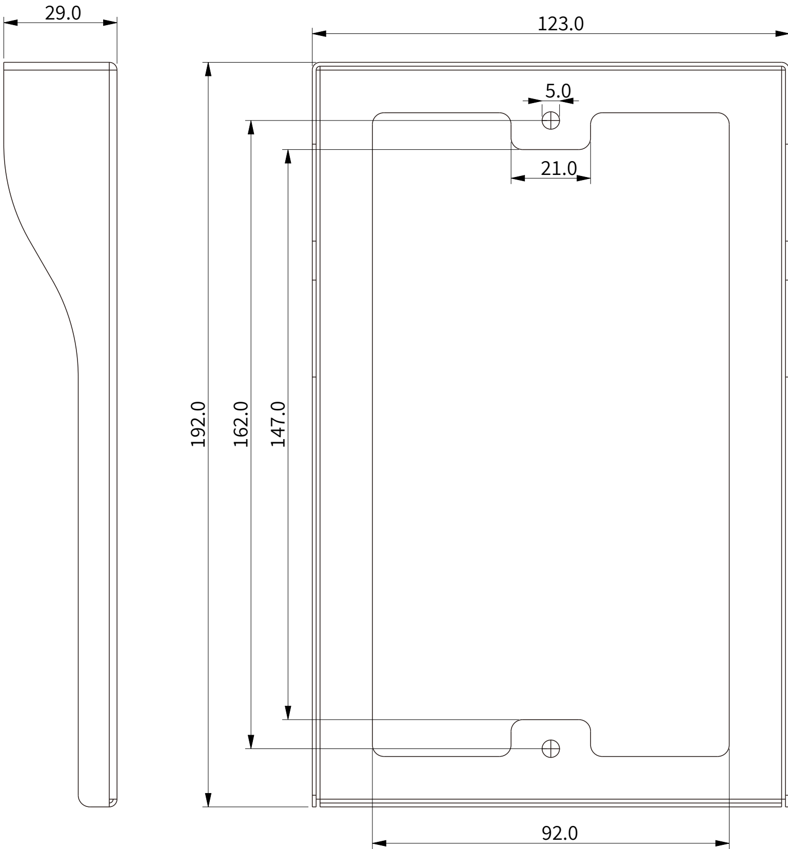
1 FRONT VIEW
