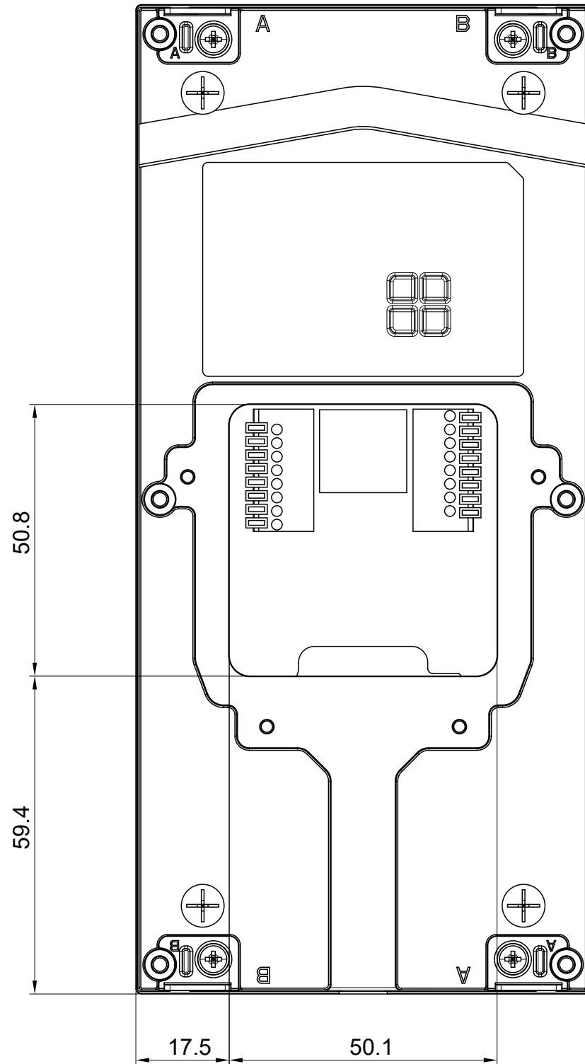
4 BACK VIEW
