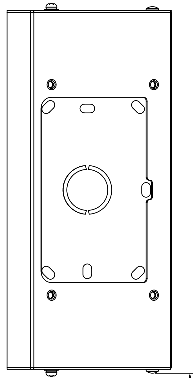
② FRONT VIEW:SLANTED WALL MOUNT BRACKET PLACEMENT
