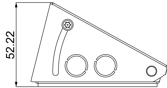
5 TOP VIEW
