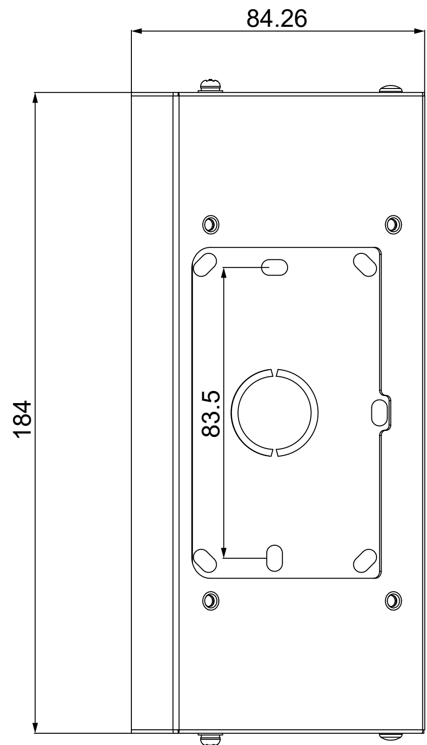
1 FRONT VIEW
