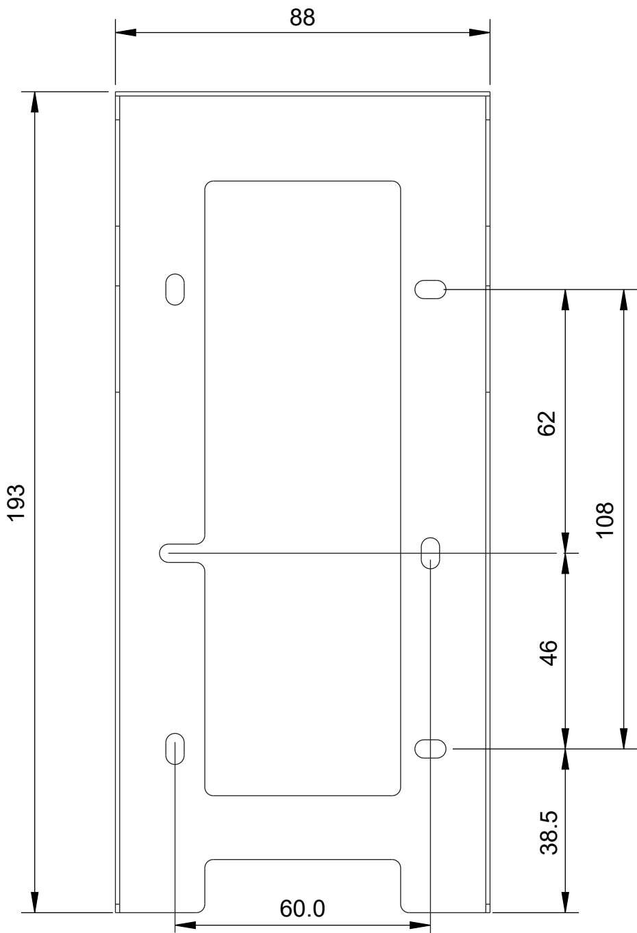
1 FRONT VIEW
