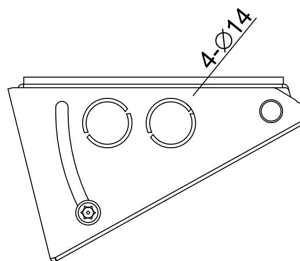
6 BOTTOM VIEW
