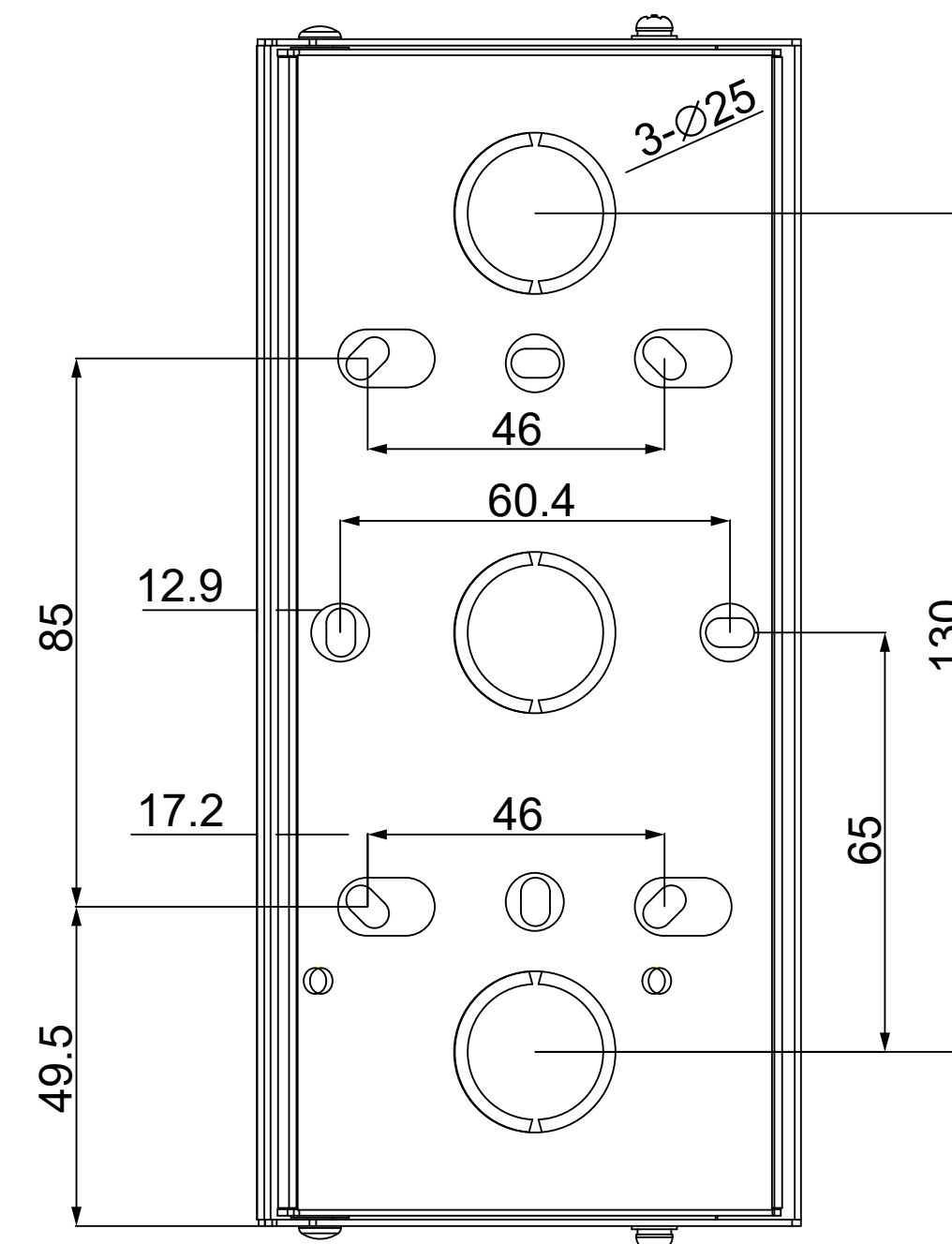
4 BACK VIEW
