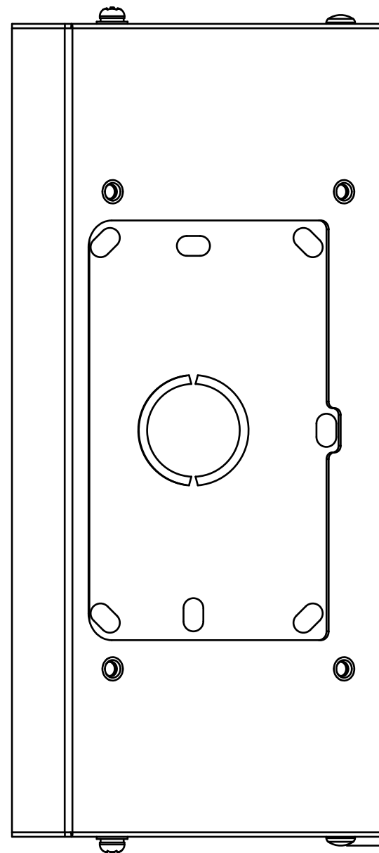
2 FRONT VIEW:SLANTED WALL MOUNT BRACKET PLACEMENT
