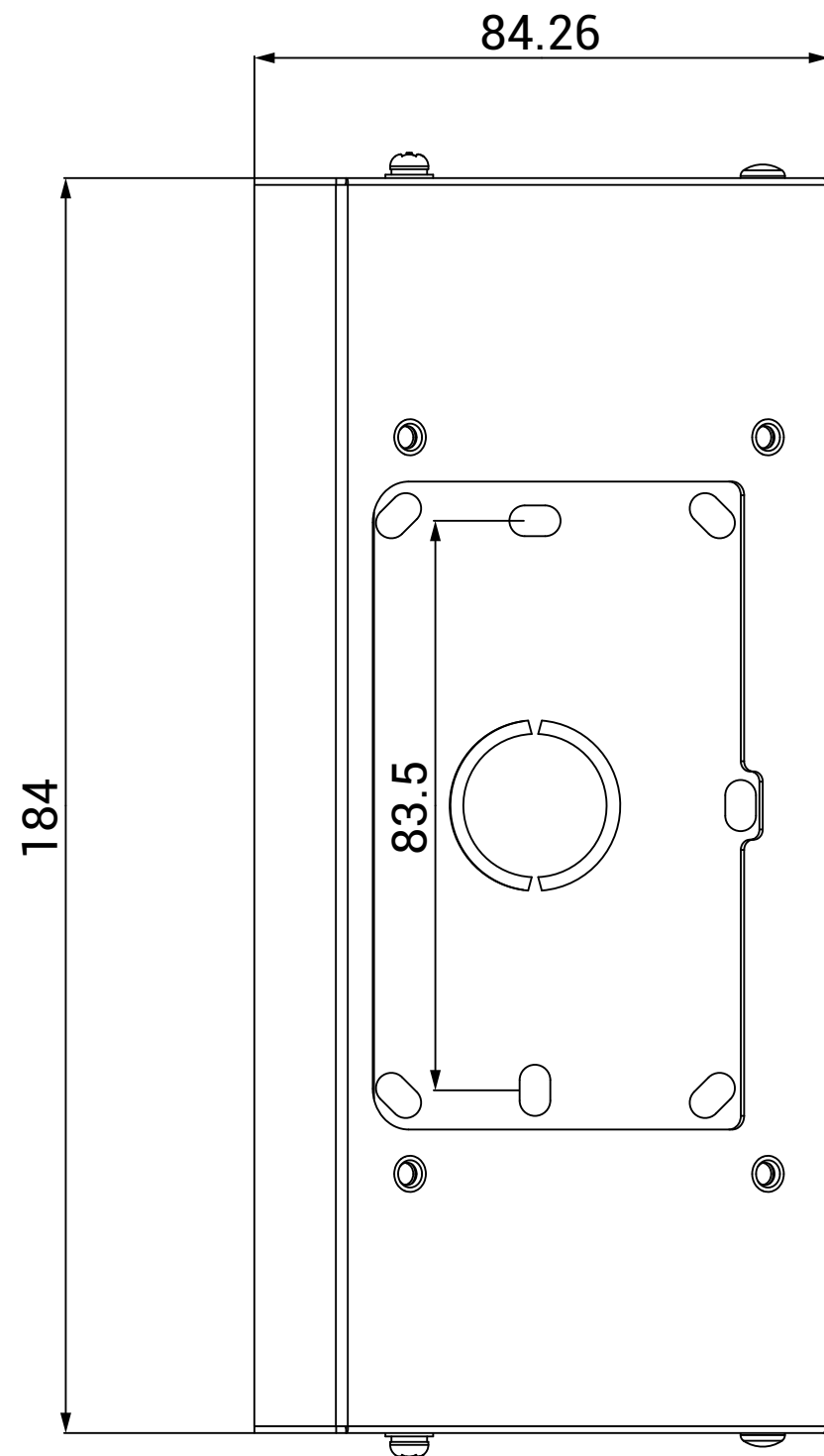
1 FRONT VIEW
