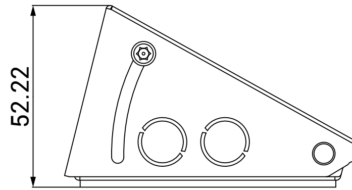
5 TOP VIEW
