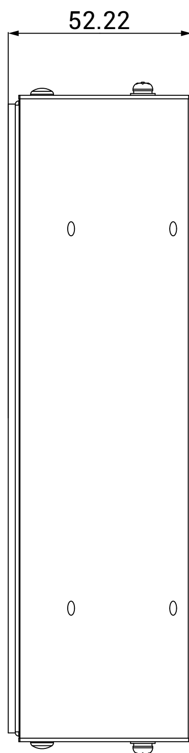
3 LEFT VIEW
