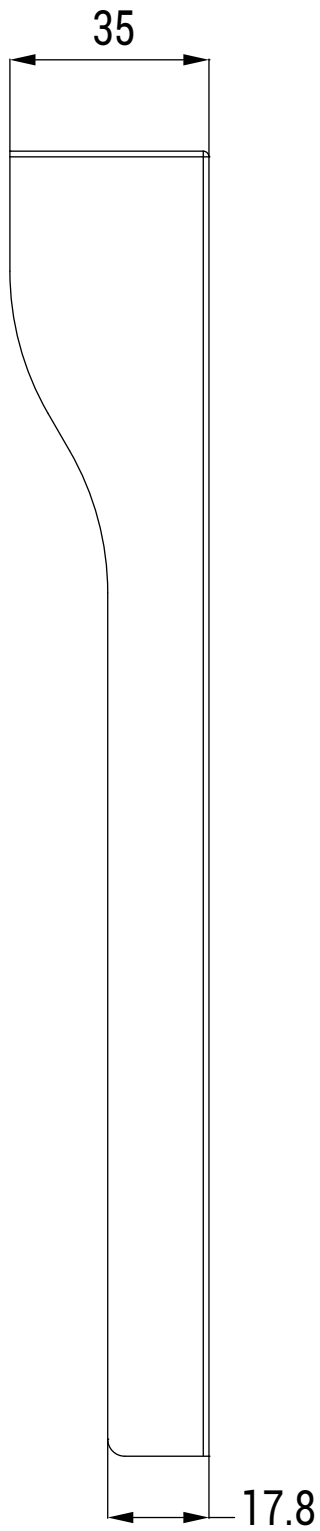
2 RIGHT VIEW
