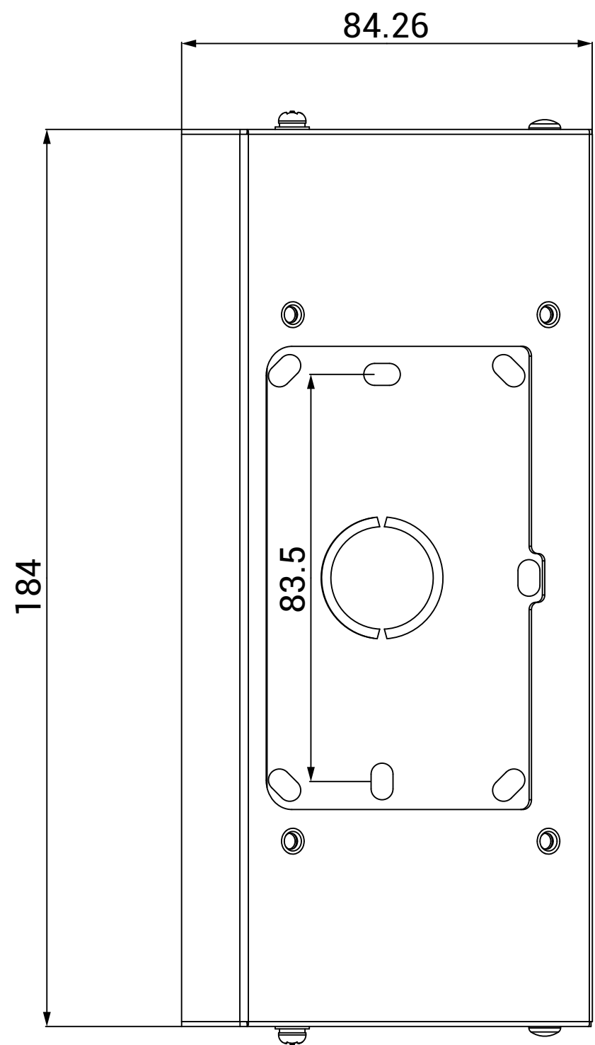
1 FRONT VIEW
