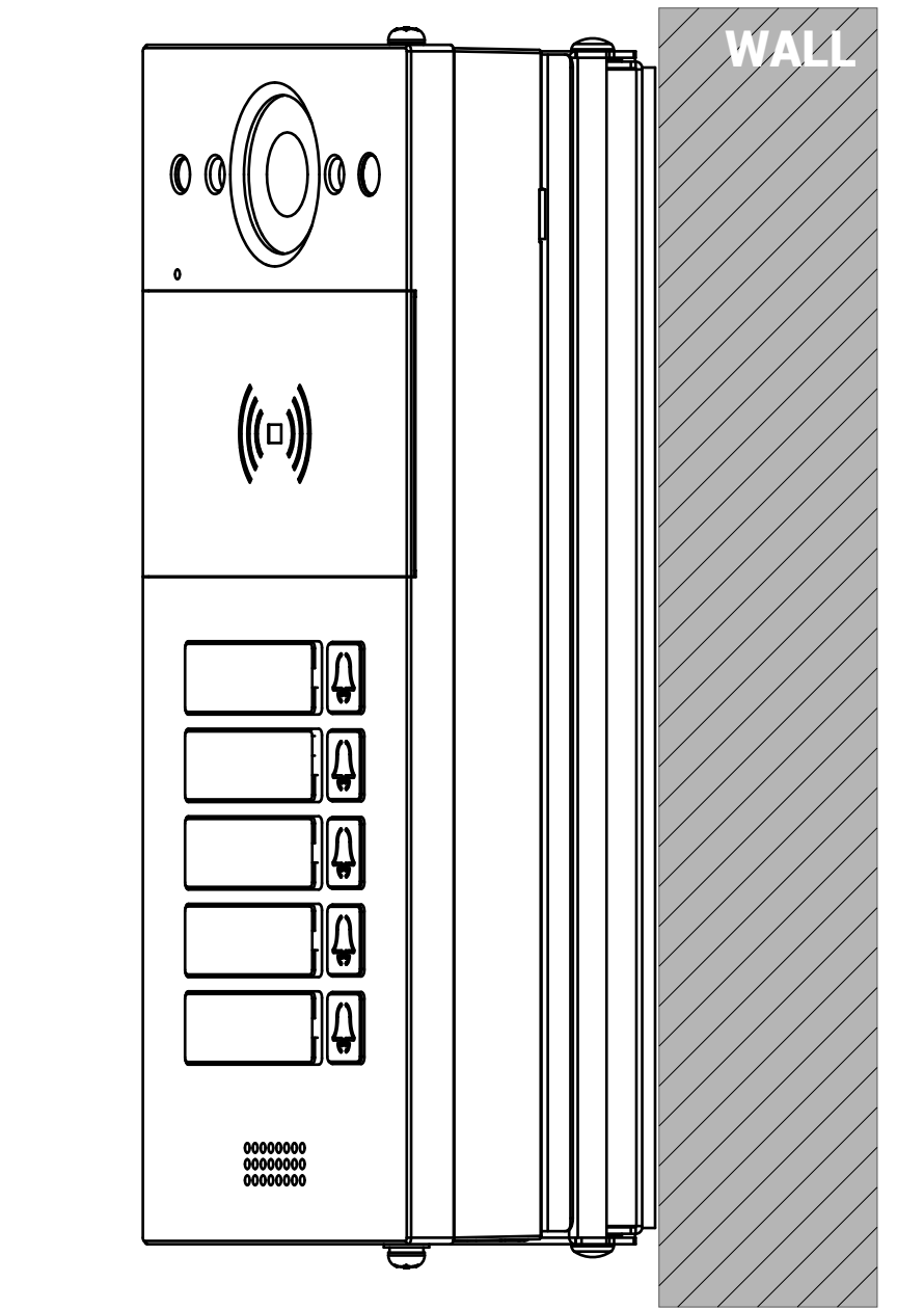
3 SIDE VIEW: INTERCOM PANEL ON WALL
