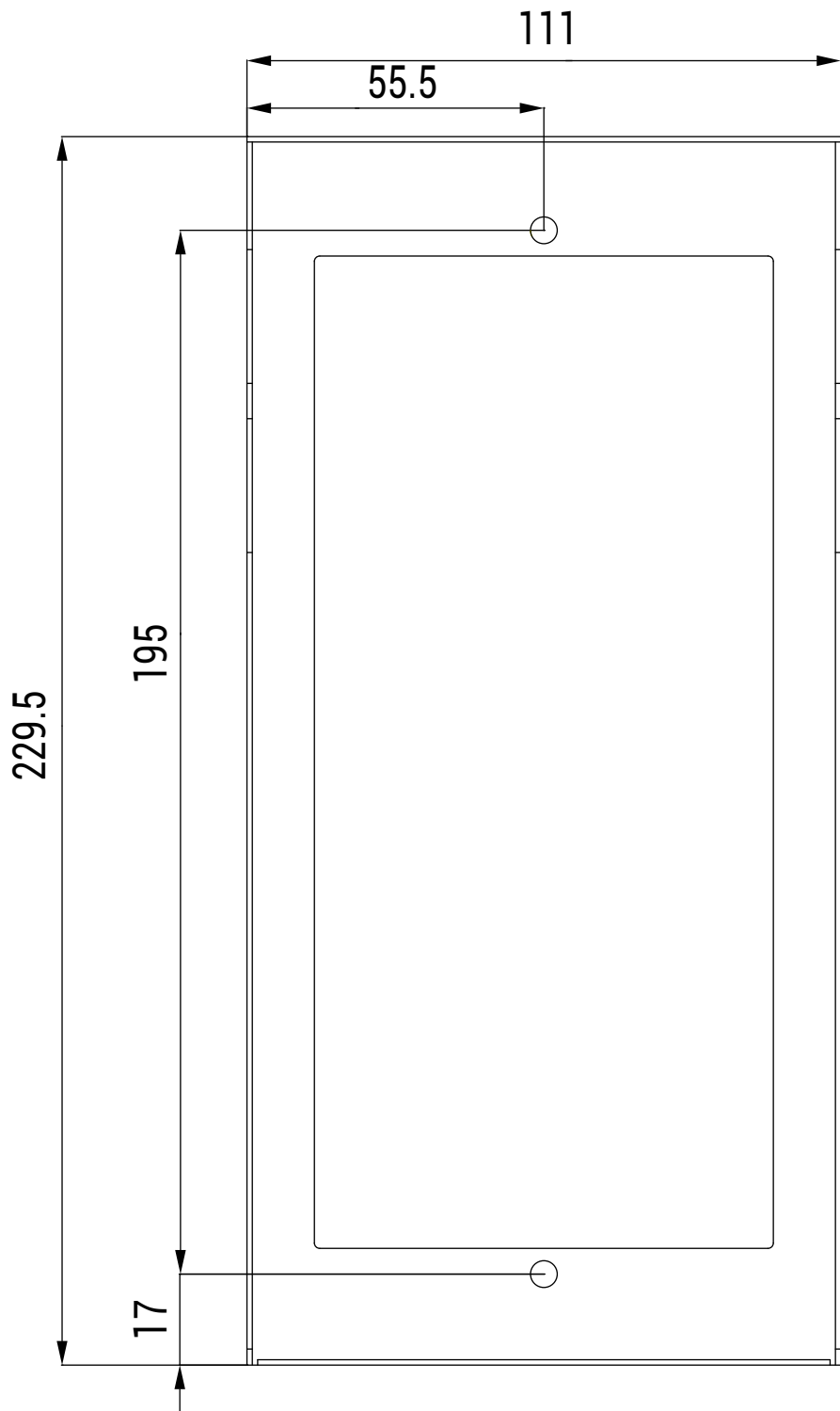
1 FRONT VIEW
