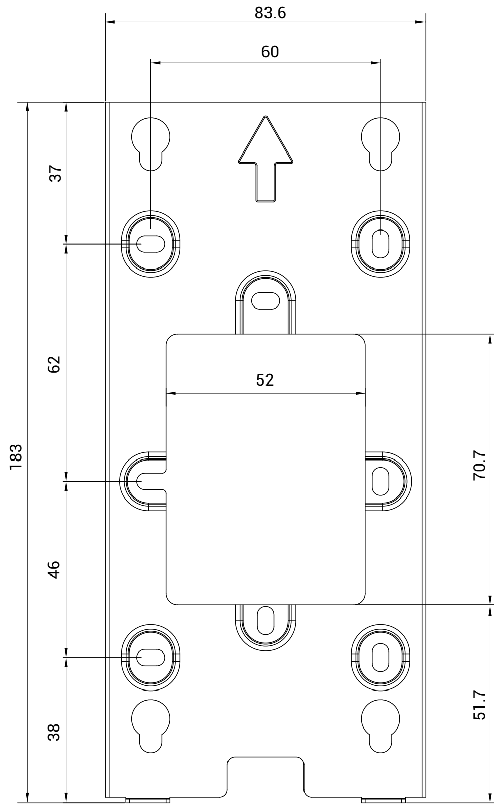
5 TOP VIEW
