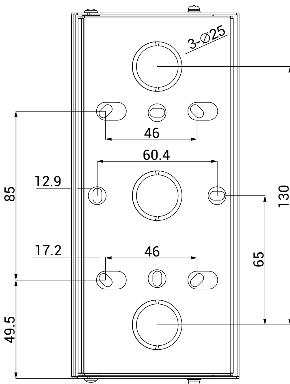
4 BACK VIEW
