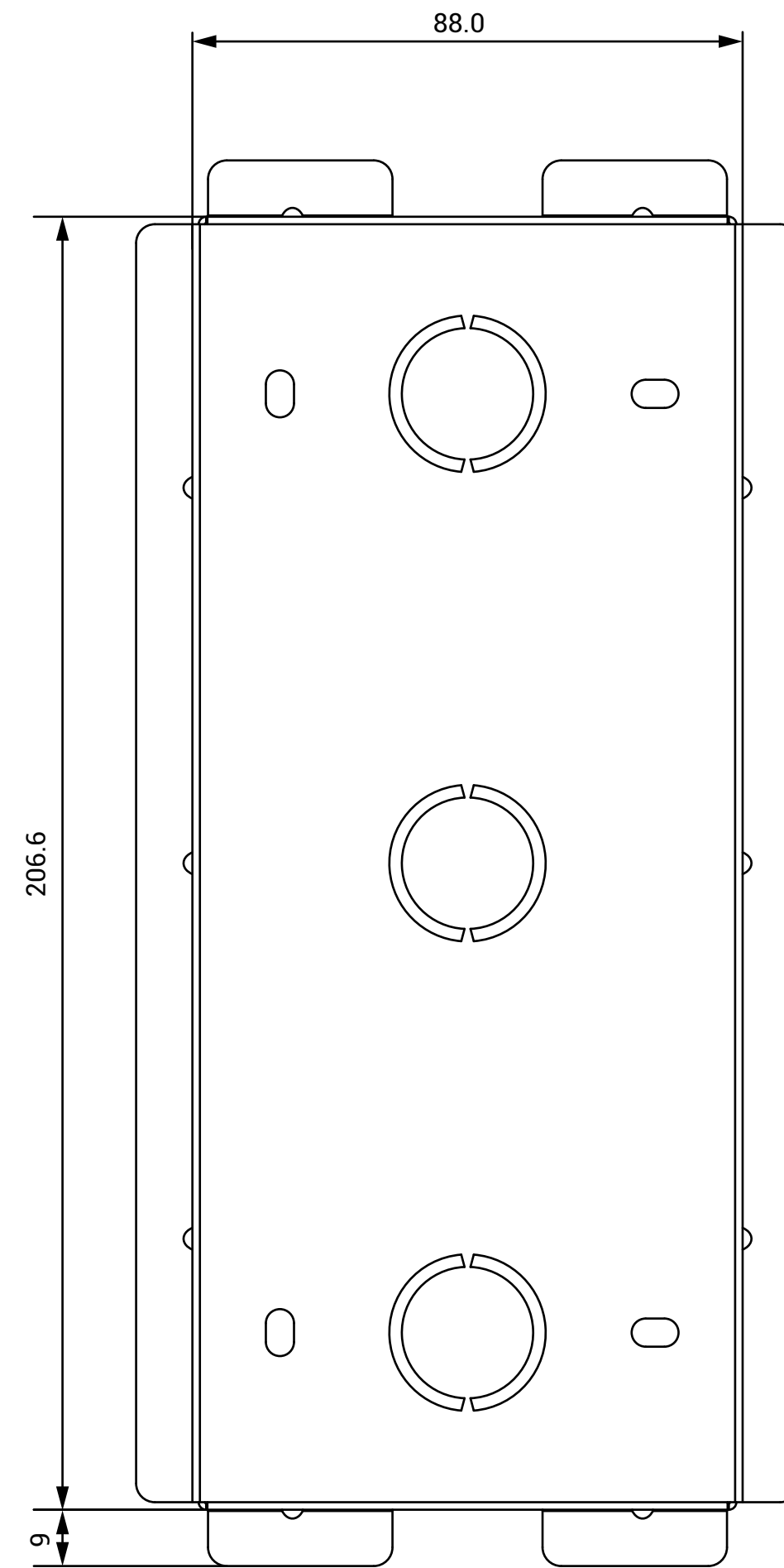
④ BACK VIEW
