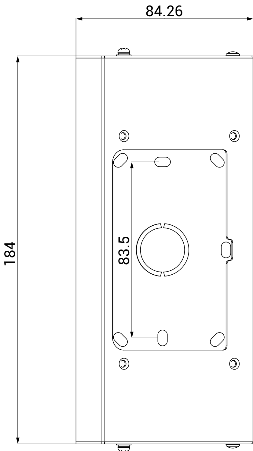
1 FRONT VIEW
