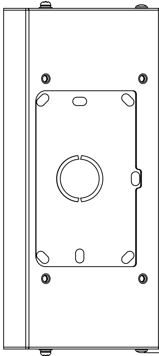
② FRONT VIEW:SLANTED WALL MOUNT BRACKET PLACEMENT
