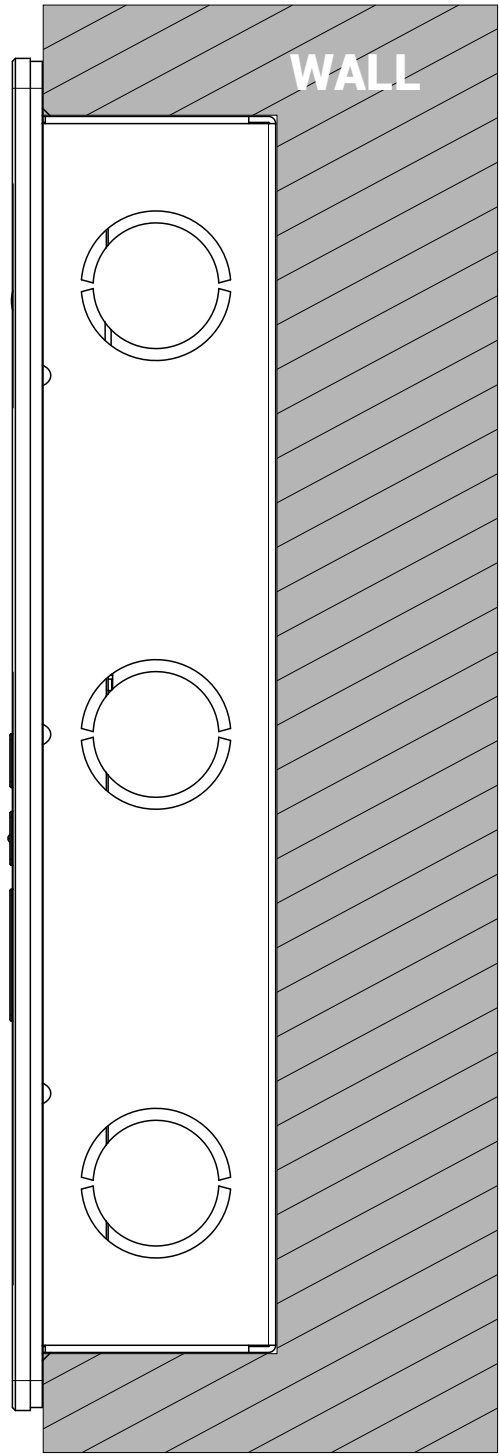
③ SIDE VIEW:INTERCOM PANEL IN WALL
