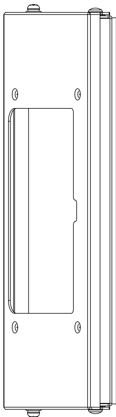
2 RIGHT VIEW
