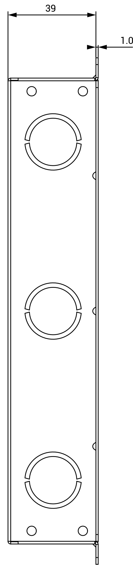
③ LEFT VIEW
