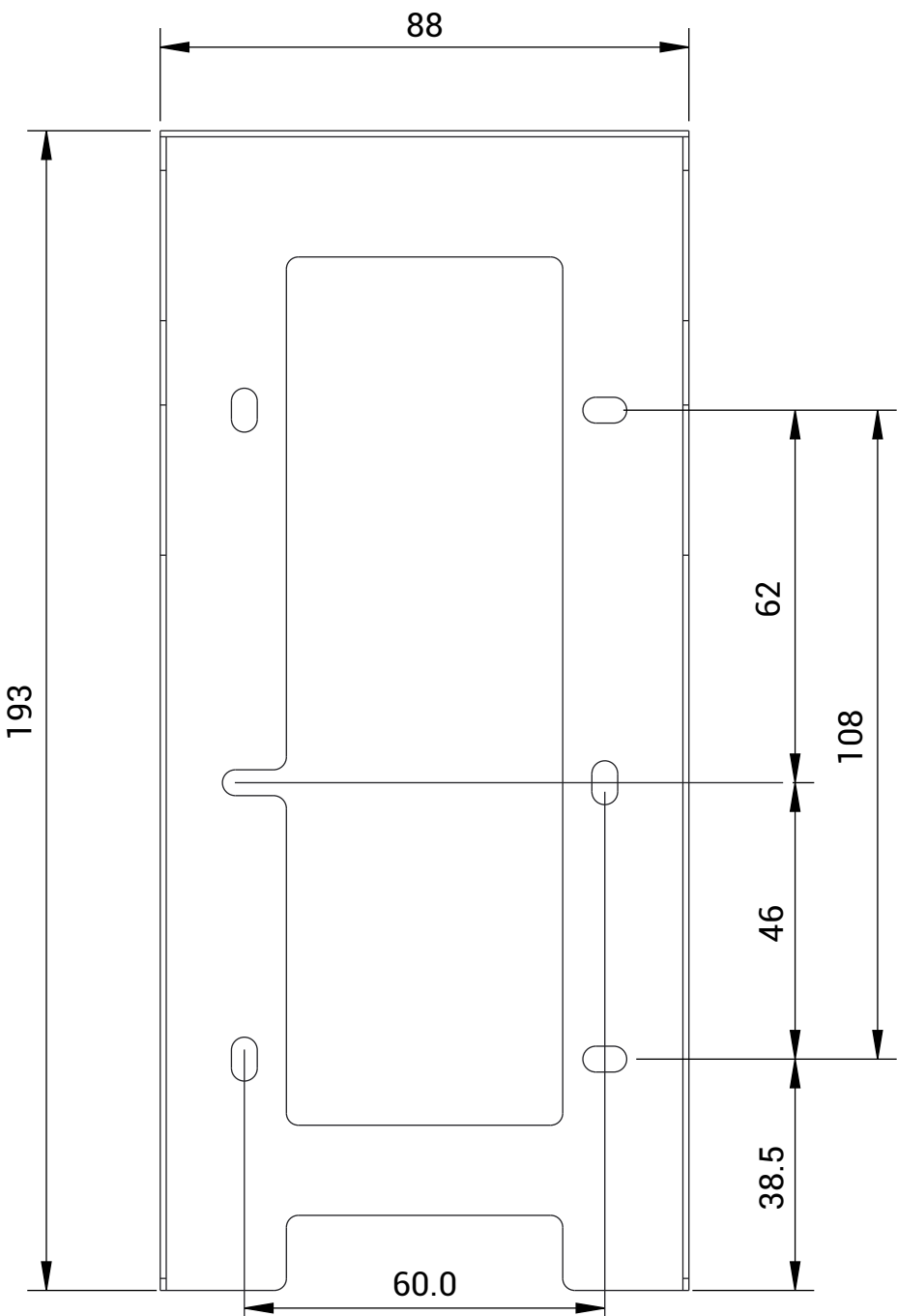
1 FRONT VIEW
