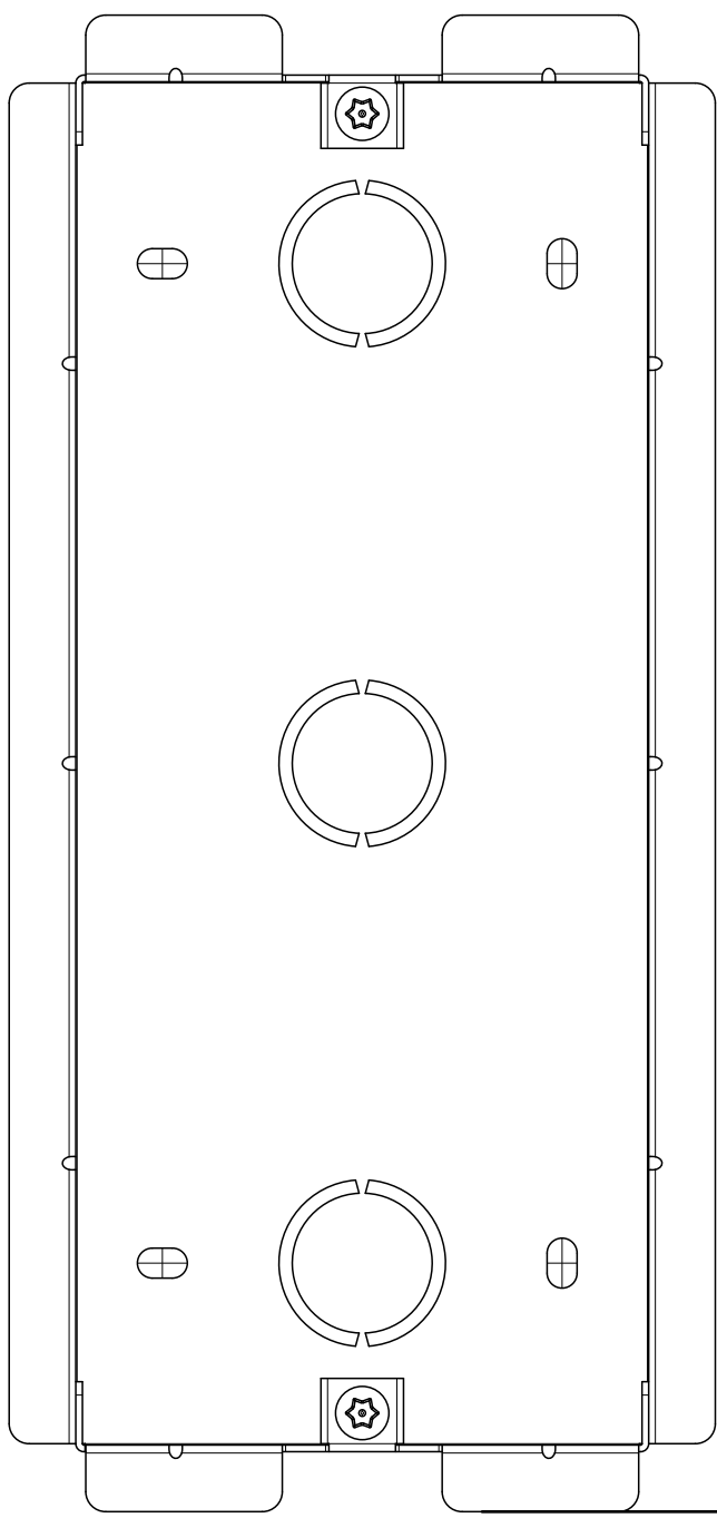
② FRONT VIEW: FLUSHING MOUNTING BOX PACEMENT
