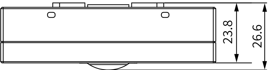
5 TOP VIEW
