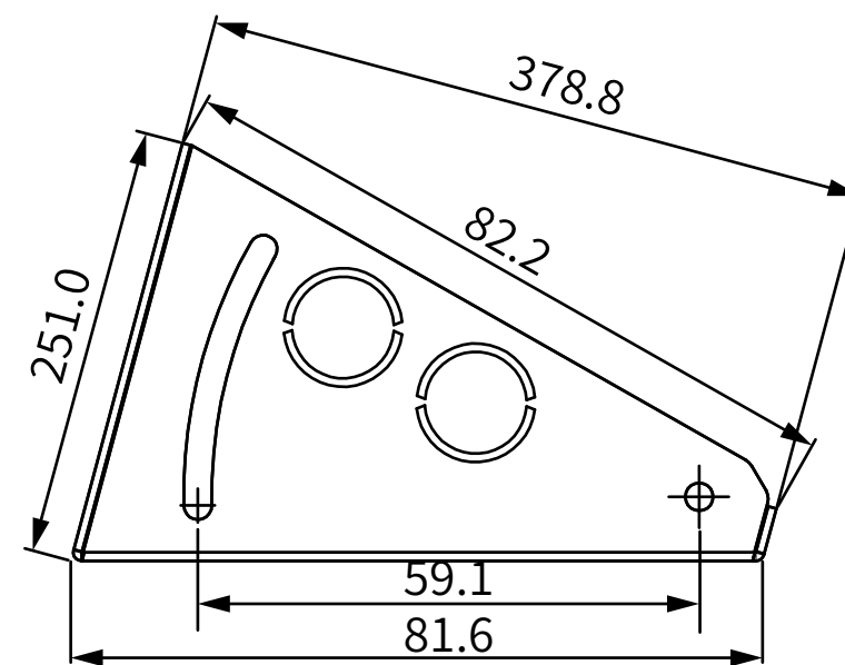
⑤ TOP VIEW
