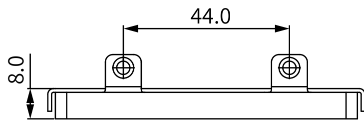
⑥ BOTTOM VIEW
