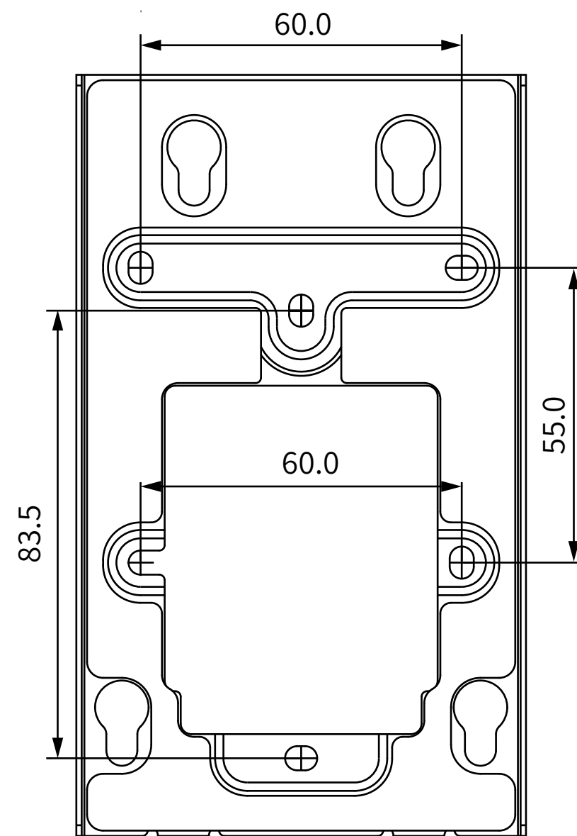
④ BACK VIEW
