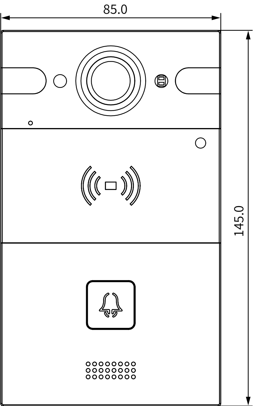
1 FRONT VIEW
