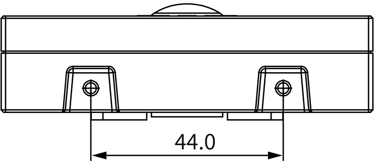
6 BOTTOM VIEW
