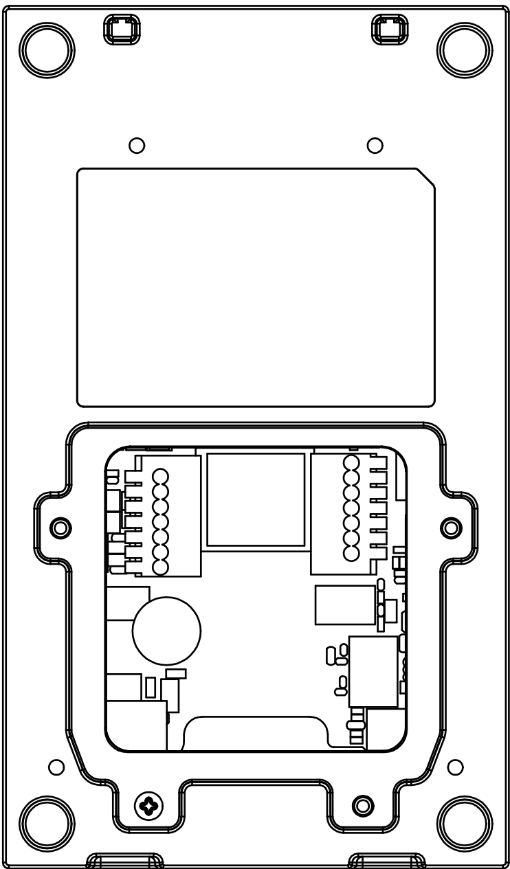
4 BACK VIEW
