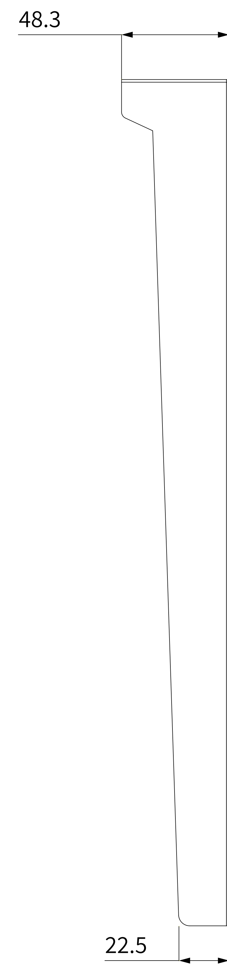
② RIGHT VIEW
