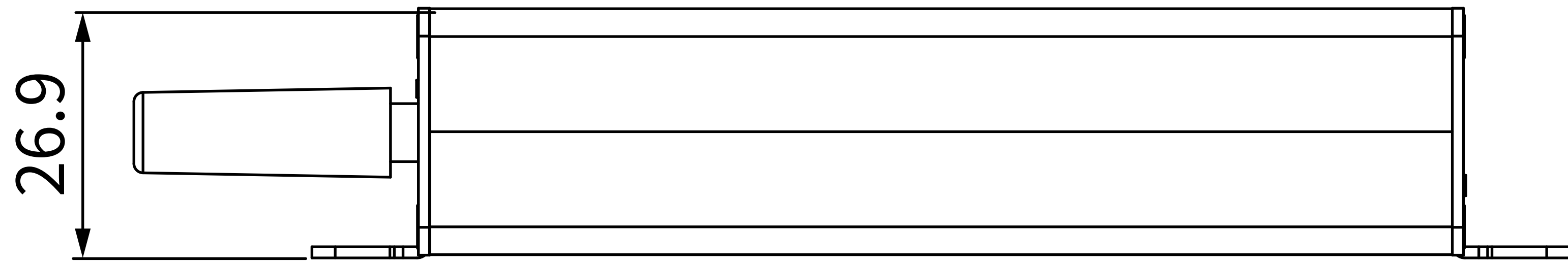
6 BOTTOM VIEW
