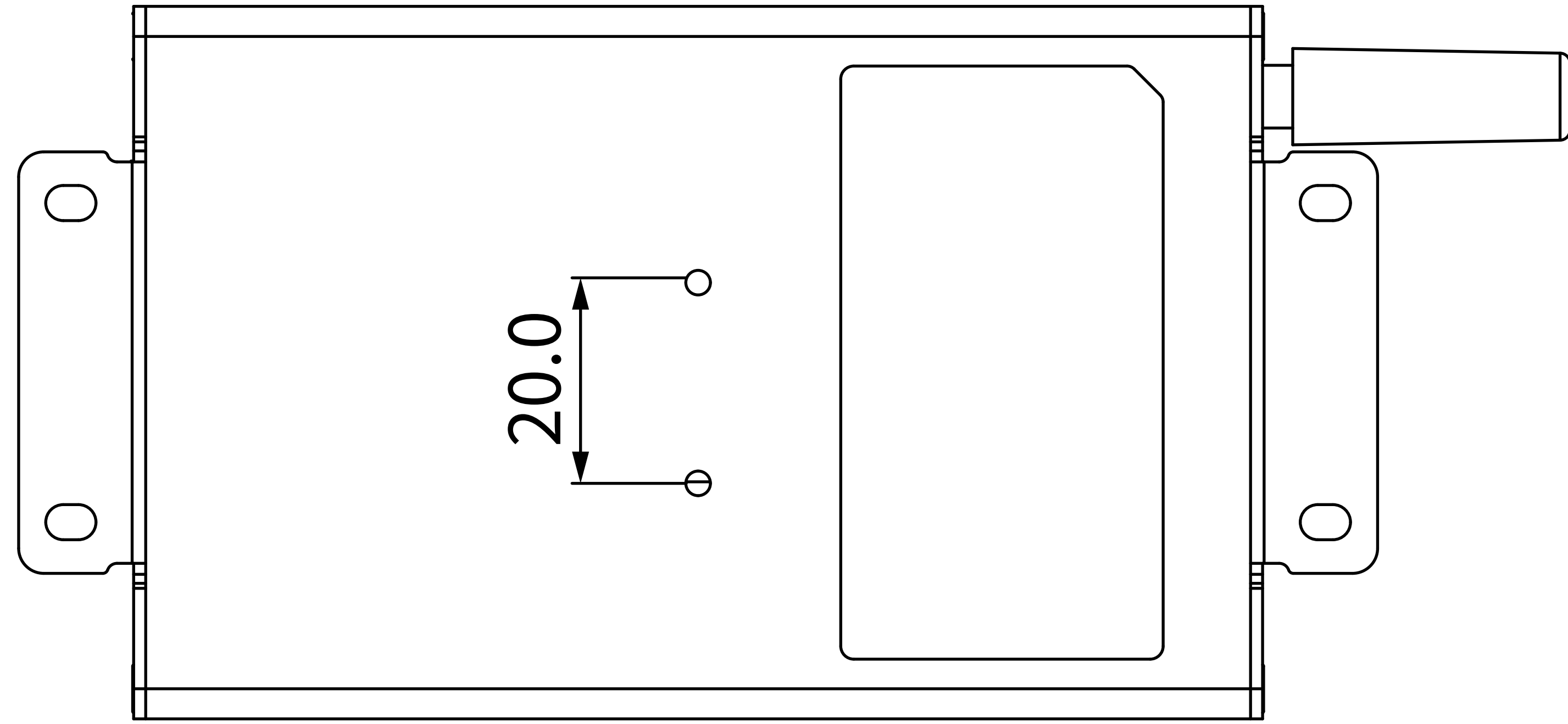
4 BACK VIEW
