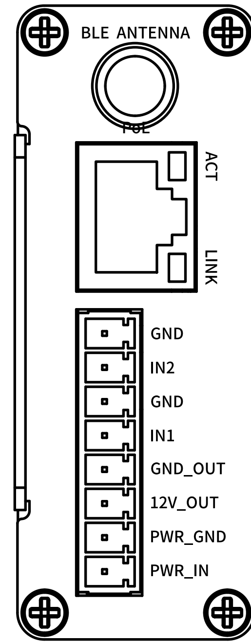
3 LEFT VIEW
