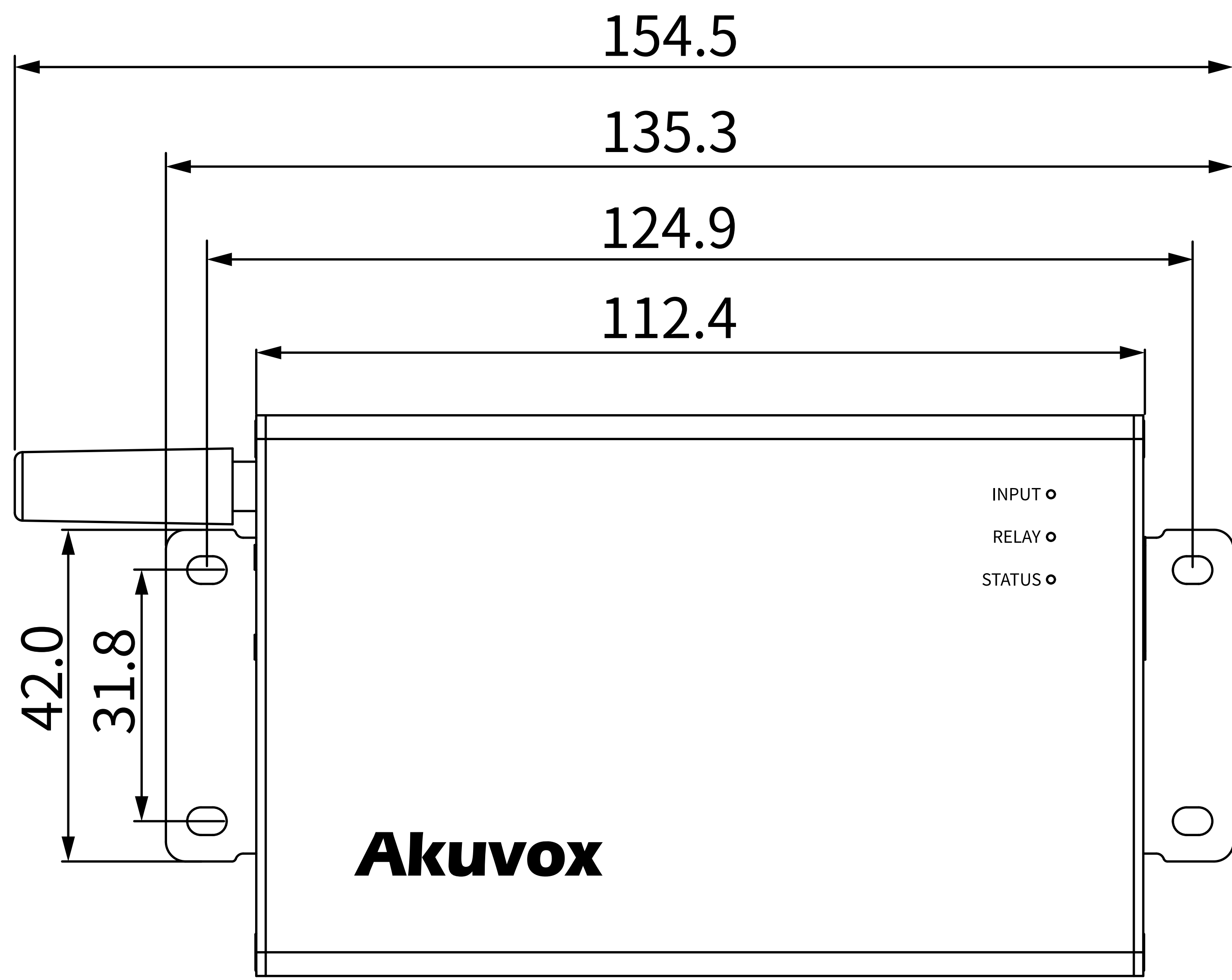
1 FRONT VIEW
