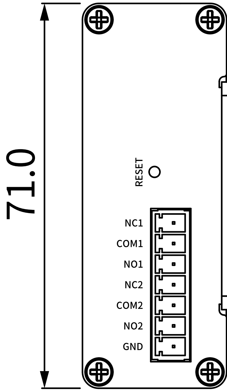
2 RIGHT VIEW
