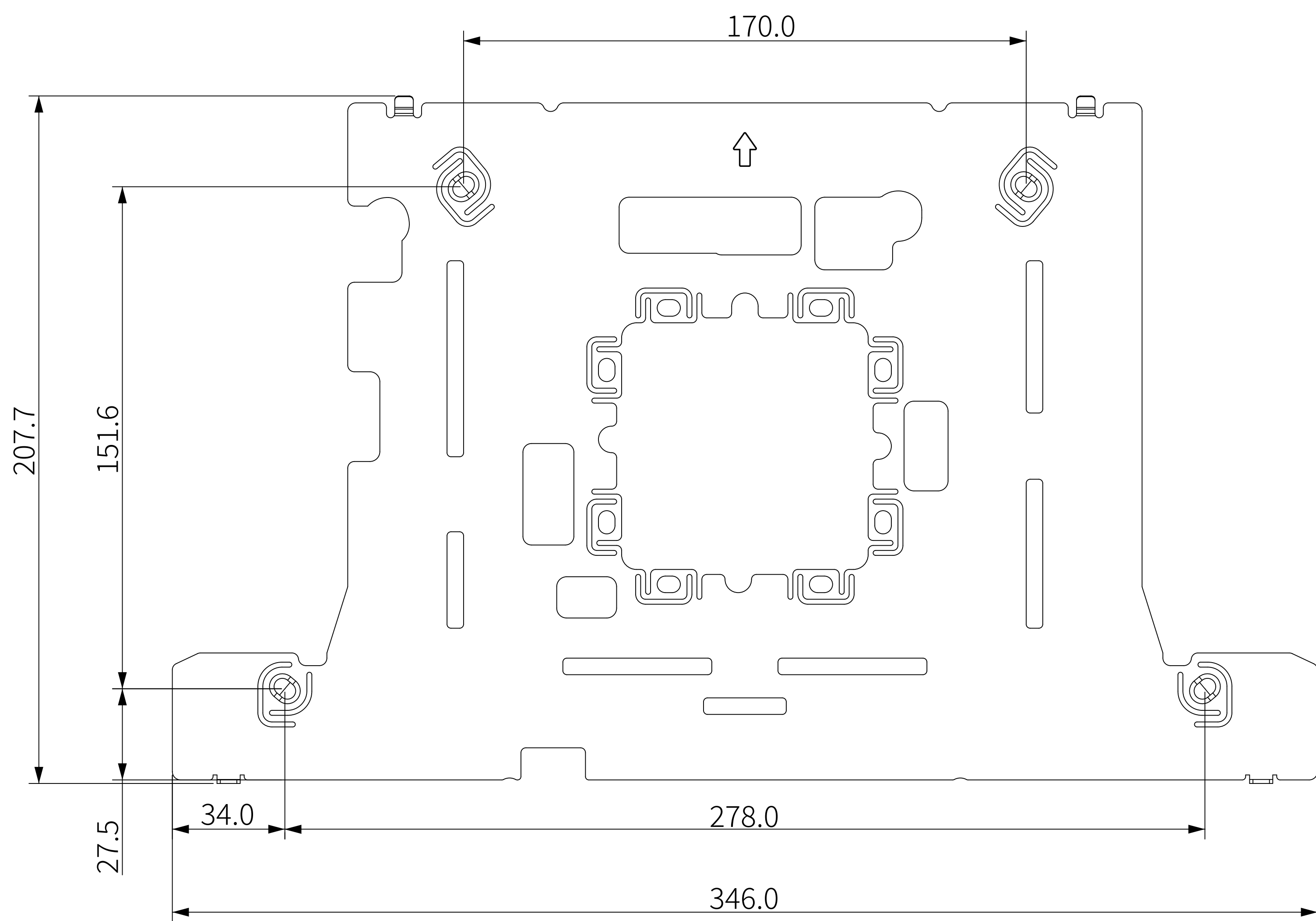
1 FRONT VIEW
