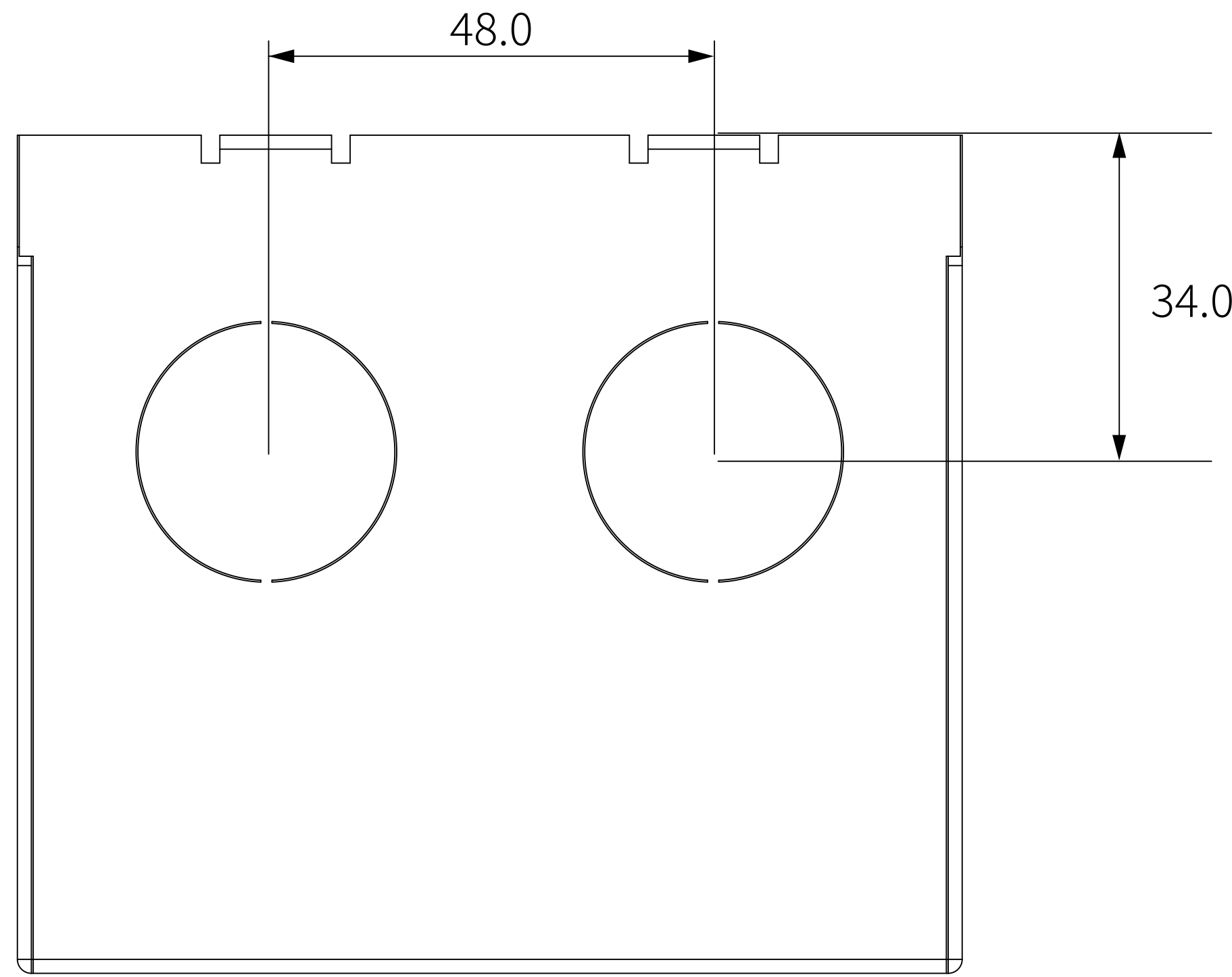
6 BOTTOM VIEW
