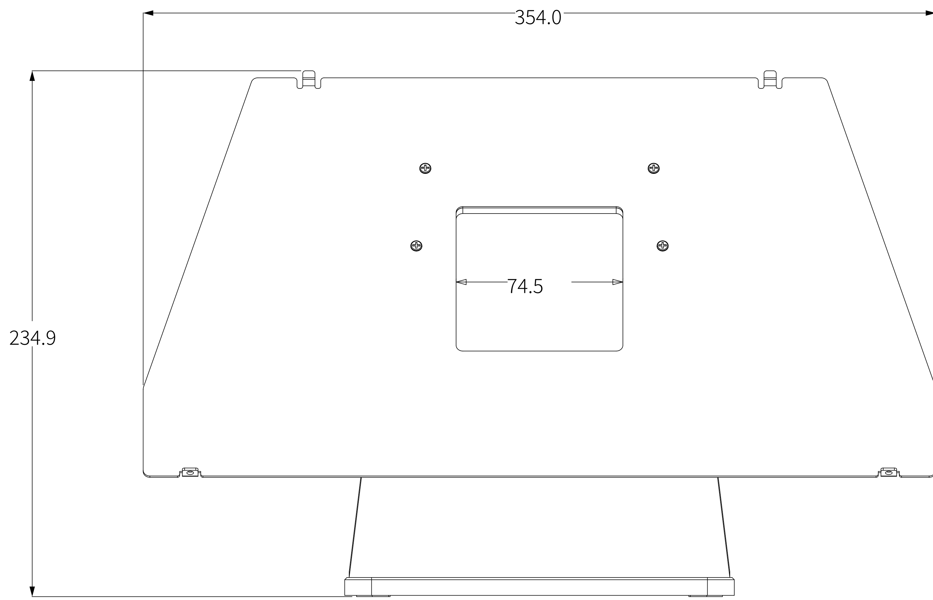
1 FRONT VIEW
