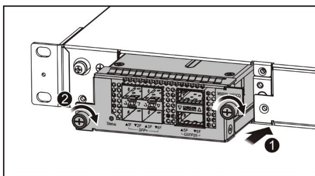
Figure 3-3 Installing an Expansion Module
