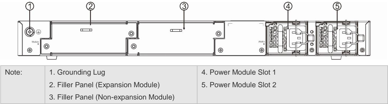
Figure 1-3 Rear Panel of RG-S5760C-24GT8XS-X
