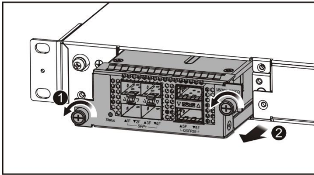
Figure 3-4 Removing an Expansion Module
