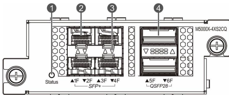
Figure 1-22 Front Panel of M5000X-4XS2CQ Module
