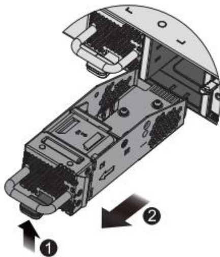
Figure 3-6 Removing a Fan Module
