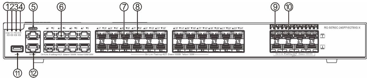
Figure 1-10 Front Panel of RG-S5760C-24SFP/8GT8XS-X
