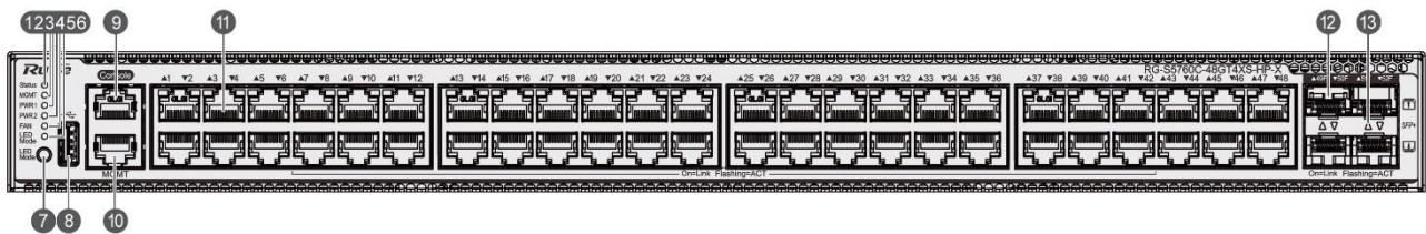
Figure 1-14 Front Panel of RG-S5760C-48GT4XS-HP-X
